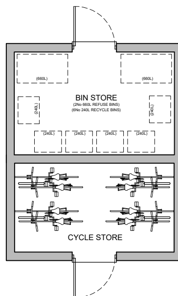
FLOOR PLAN
