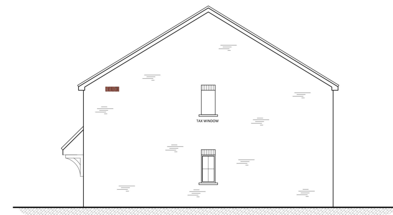
SIDE ELEVATION
