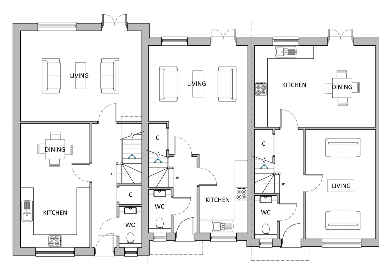
PLOT 8 PLOT 7 PLOT 6 GROUND FLOOR PLAN
