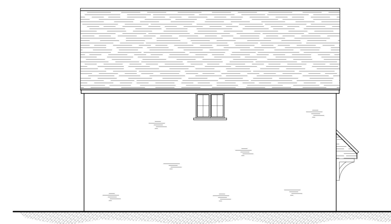
SIDE ELEVATION
