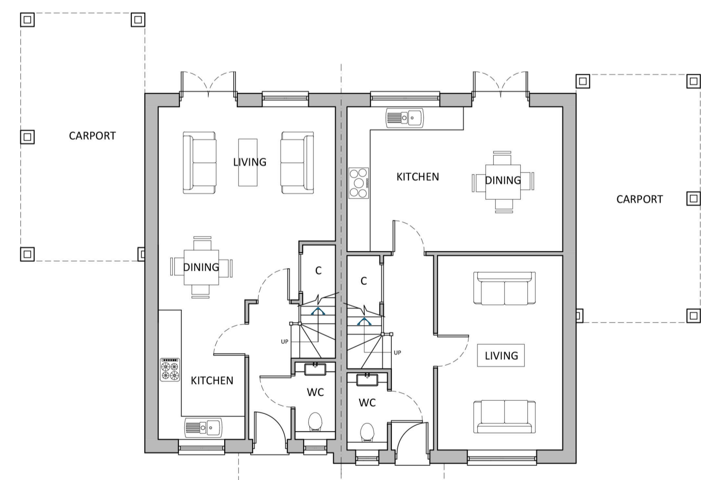
PLOT 23 PLOT 22 GROUND FLOOR PLAN
